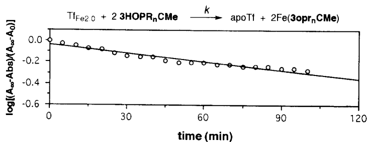
Figure 2. The plots of \log[(A_x - \text{Abs}) / (A_x - A_0)] vs time on iron removal of 3HOPR 6 CMe from Tf Fe2.0 .
